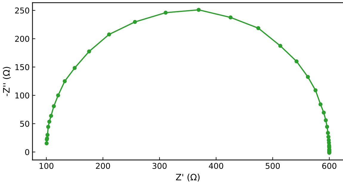
Nyquist Plot — default
