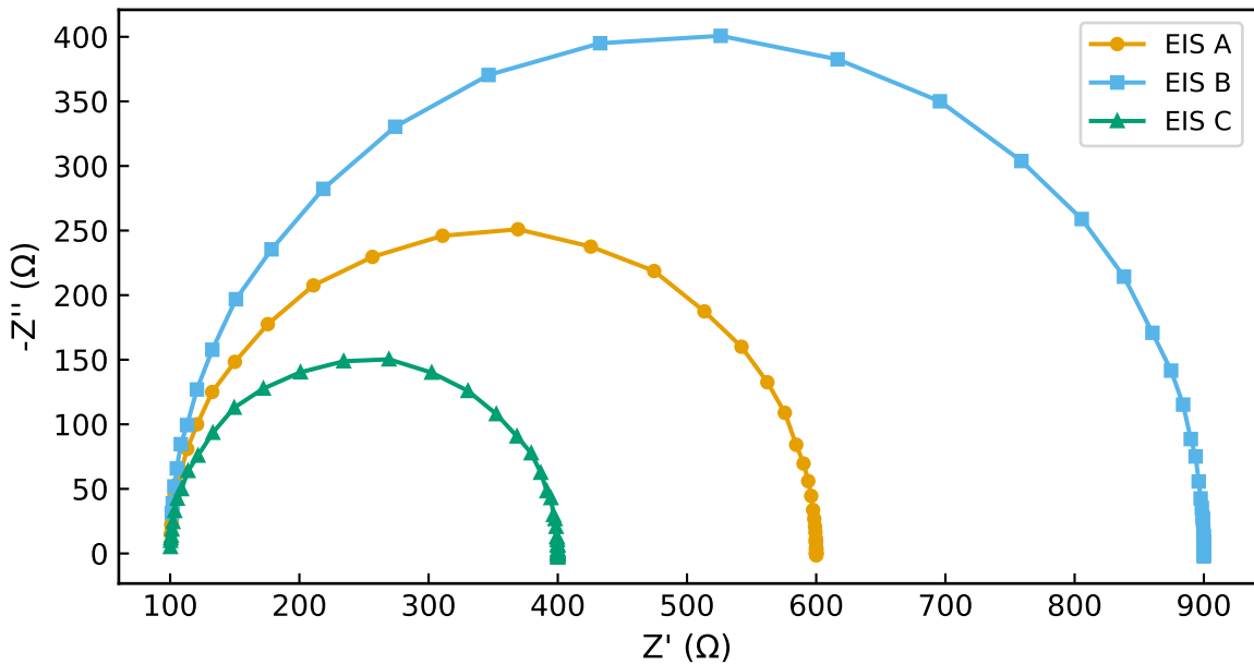
Nyquist Overlay — default
