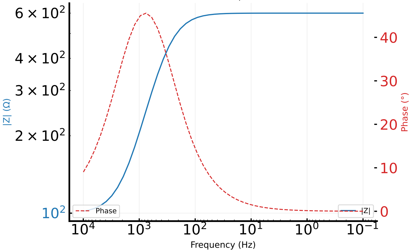
Bode Plot — poster
