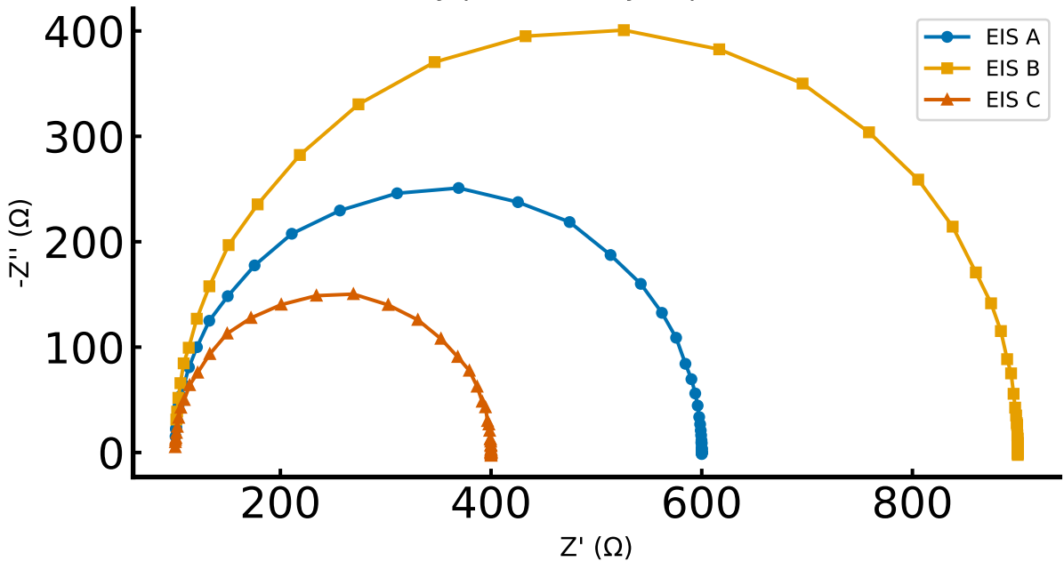
Nyquist Overlay — poster
