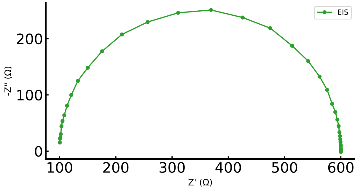
Nyquist Plot — poster
