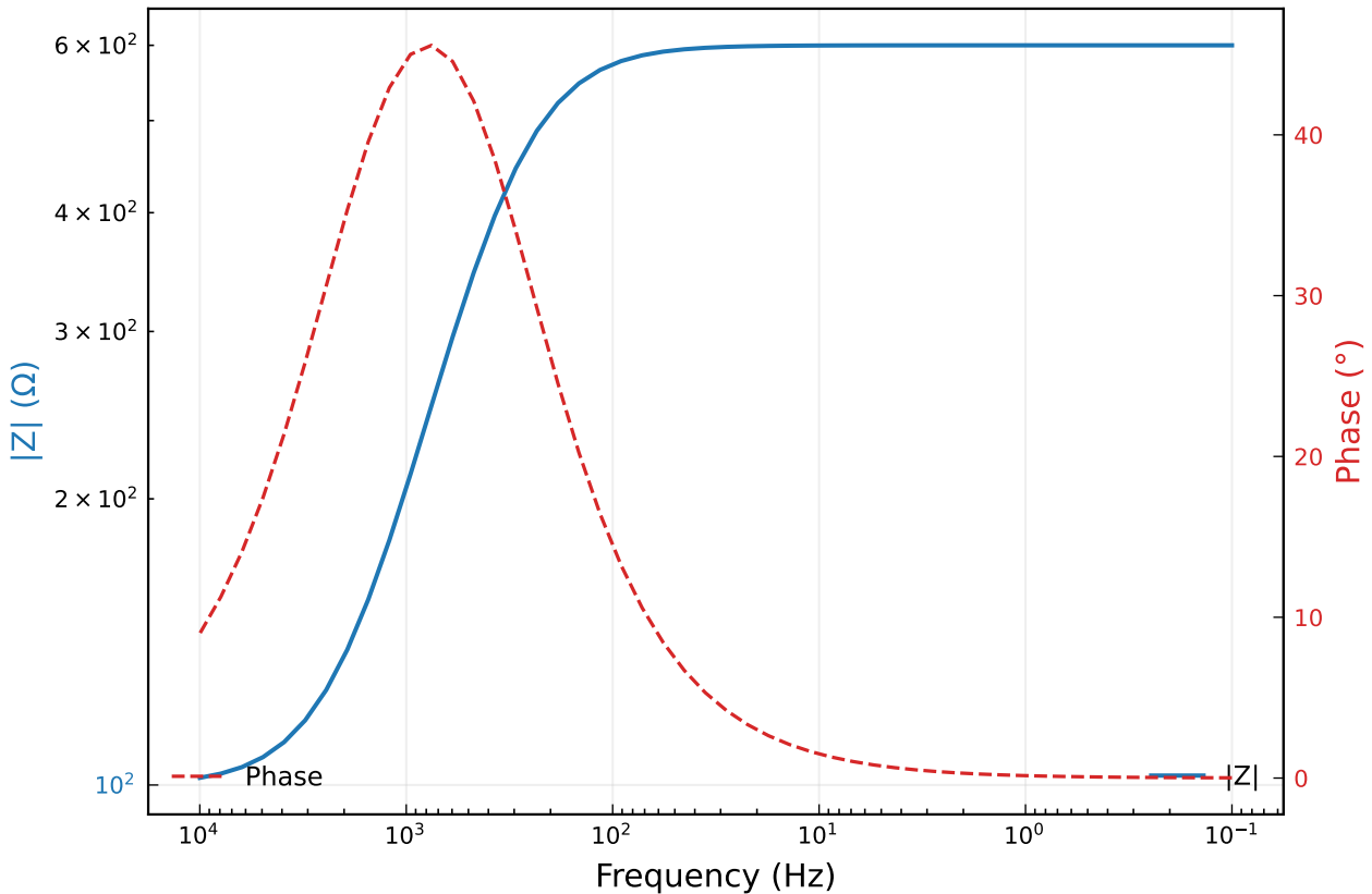
Bode Plot — publication-acsc
