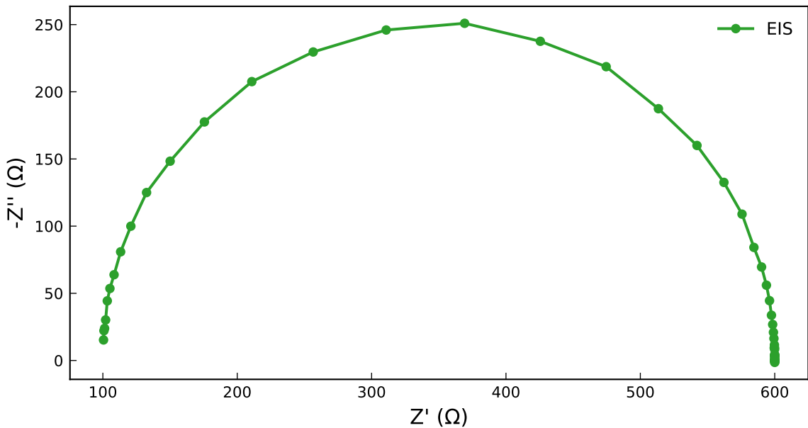
Nyquist Plot — publication-acs
