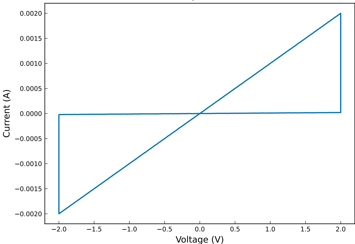
IV Curve — publication-acsc
