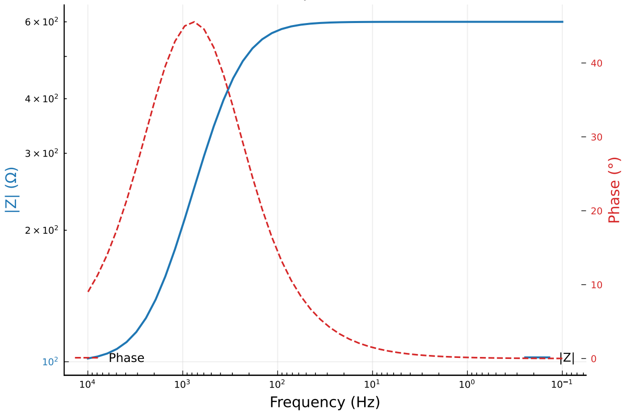
Bode Plot — publication-nature
