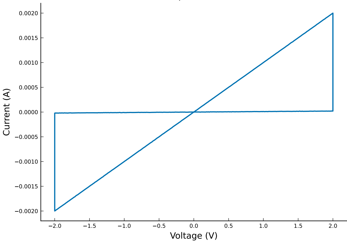
IV Curve — publication-nature
