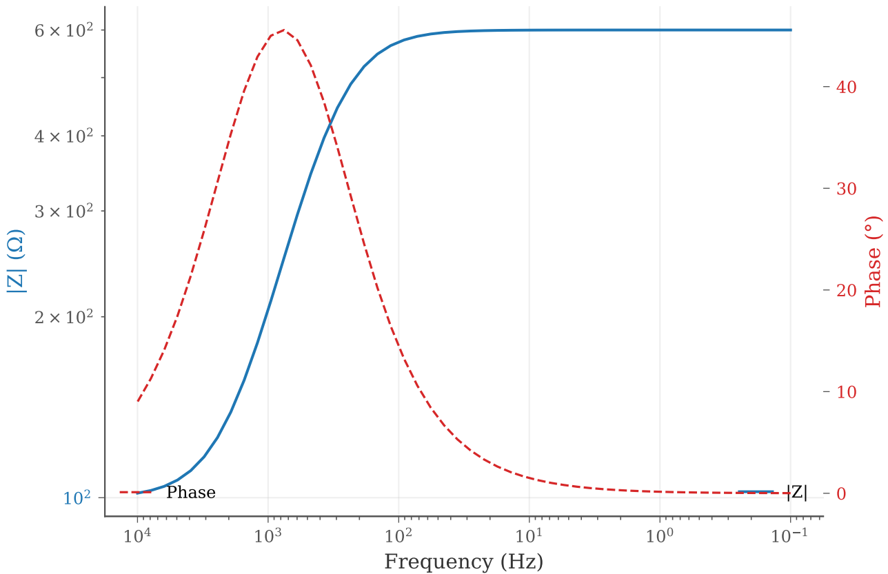
Bode Plot — tuft
