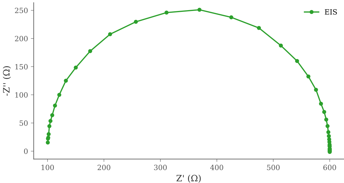
Nyquist Plot — tuftes
