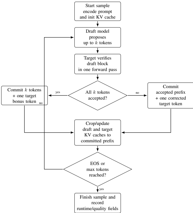
Fig. 1. Vanilla speculative decoding implementation flow used in Phases 3–4. The target model remains the verifier of record; accepted draft prefixes are committed and caches are cropped to preserve exact target-consistent decoding.
