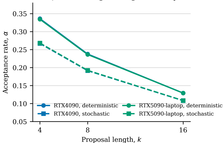
(c) Qwen3 acceptance portability
