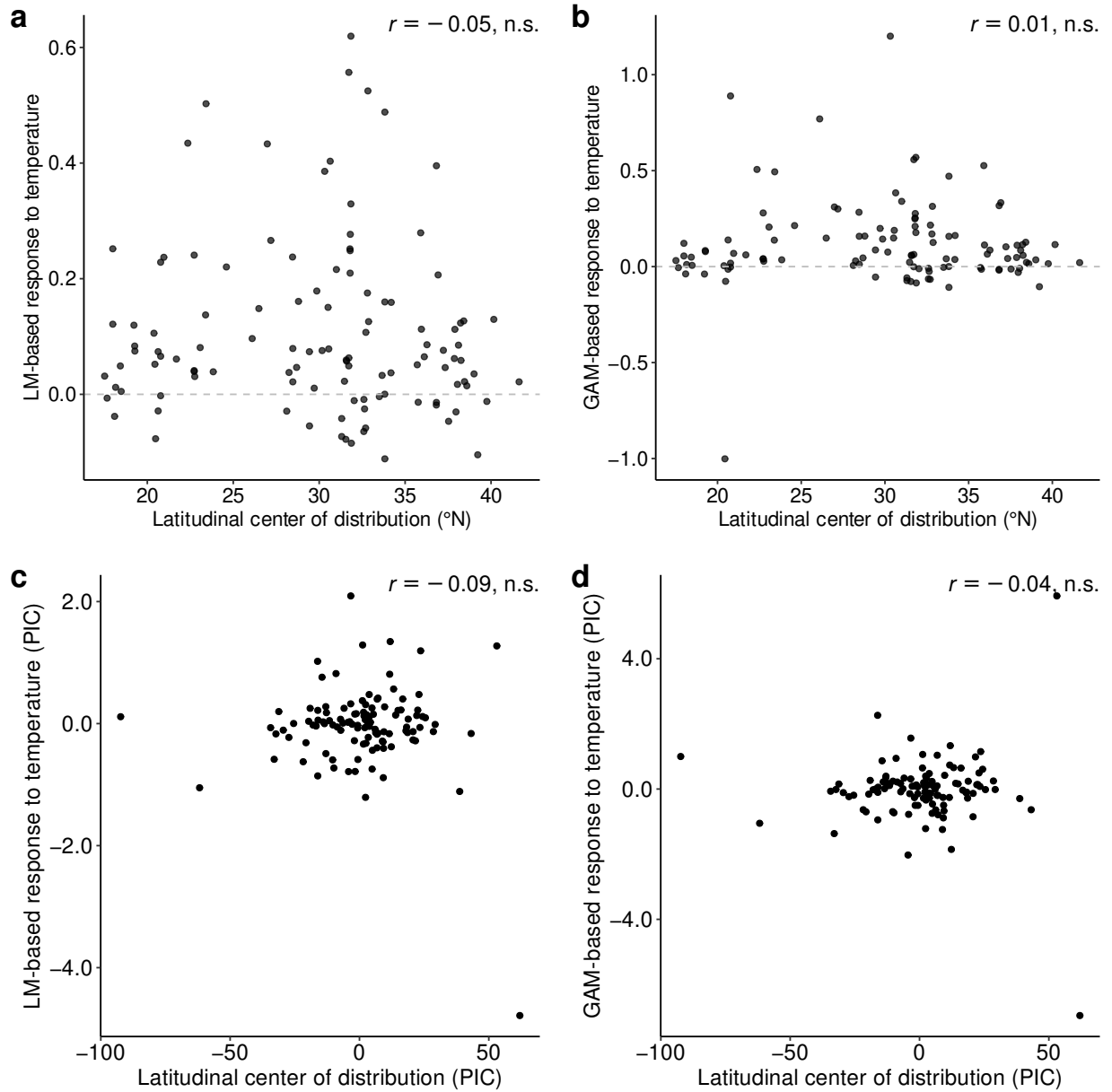
Extended Data Figure 3 | Relationships between latitudinal distribution and conventional temperature response traits. Relationships between species' latitudinal distribution centers and their temperature responses estimated by linear model (LM) or generalized additive model (GAM). a , Latitudinal distribution center versus LM-based response (slope of the linear model between temperature and abundance). b , Latitudinal distribution center versus GAM-based response (mean slope of the first derivative of the fitted GAM). c–d , Corresponding relationships accounting for phylogenetic relatedness using phylogenetic independent contrasts (PIC). The Pearson's correlation coefficient ( r ) and its p value are indicated in the figure.
