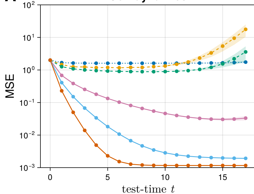
CoT dynamics
