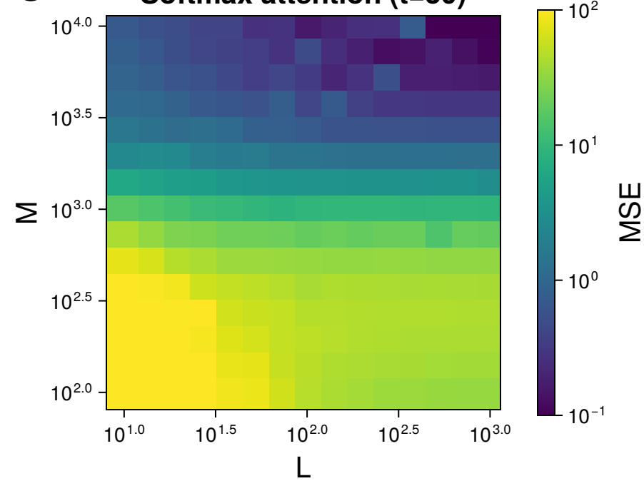
Softmax attention (t=30)
