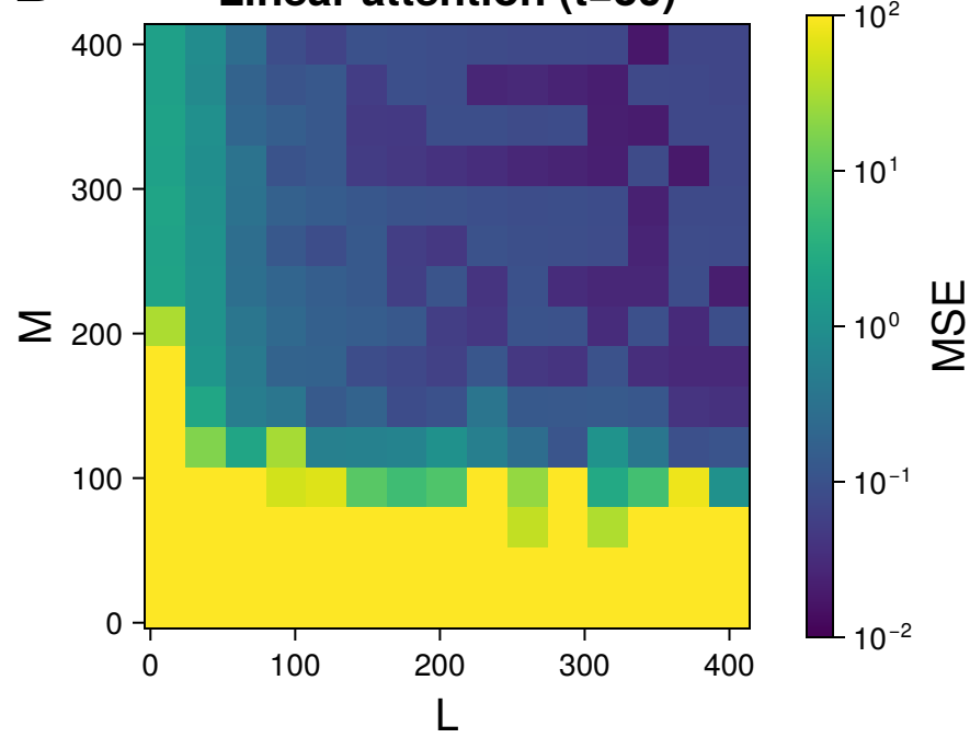
Linear attention (t=30)
