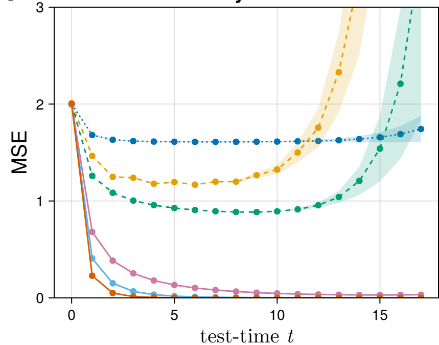
CoT dynamics
