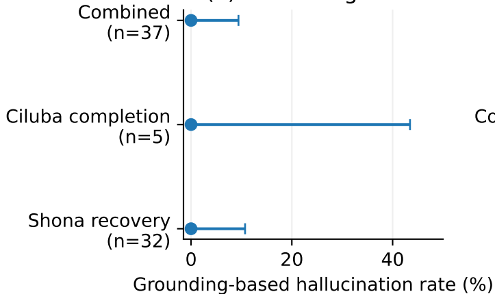
(a) Grounding audit
