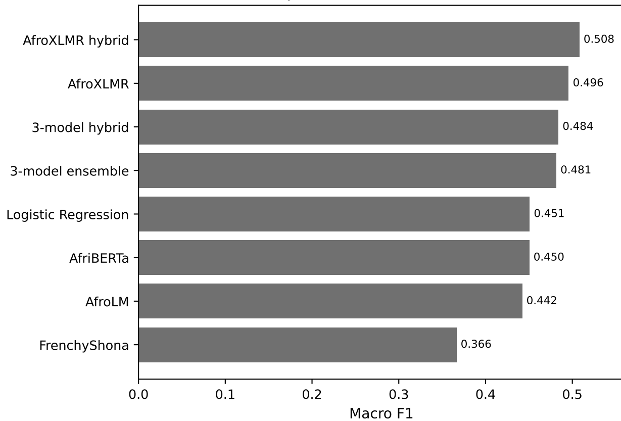
(a) Selected systems on the strict unseen Shona test
