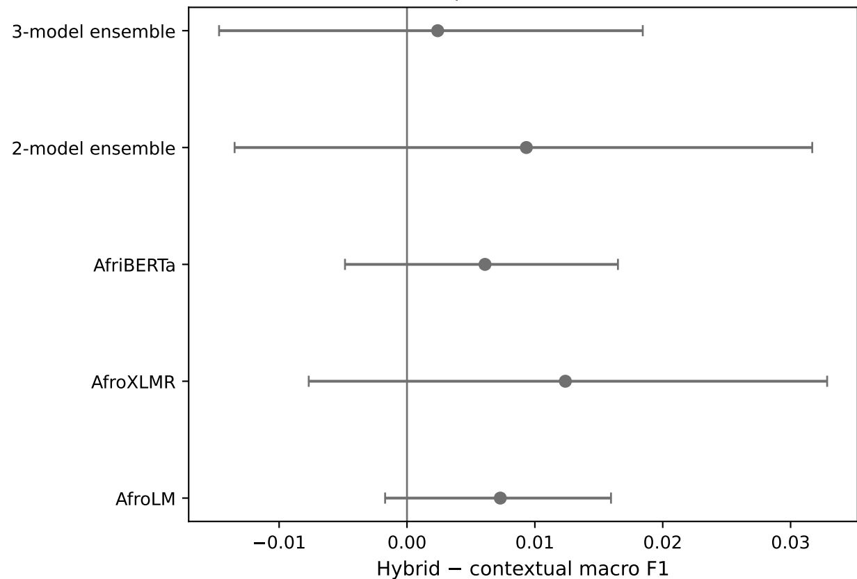
(b) Paired-bootstrap differences with 95% intervals
