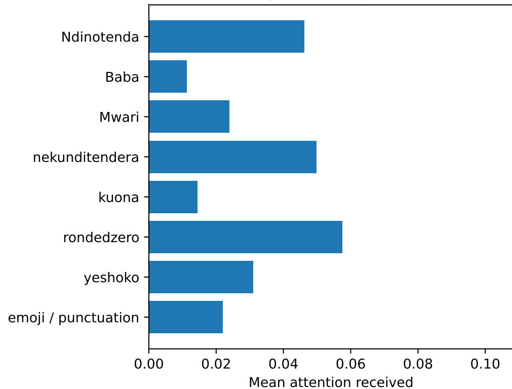
(a) AfroLM POS prediction, p=0.756
