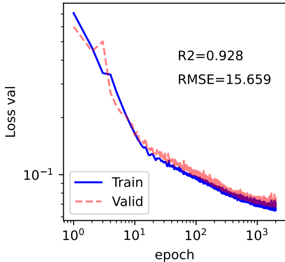
SGD, LR=0.1
