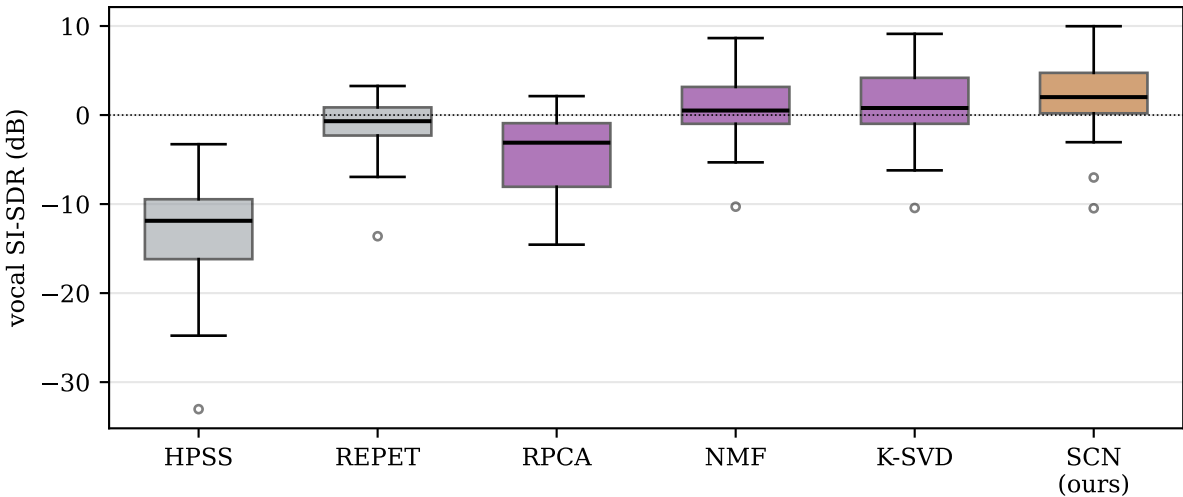
Per-track vocal SI-SDR distribution (25 tracks)
