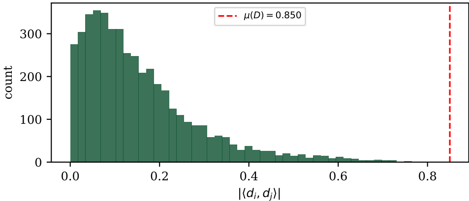
K-SVD vocal dictionary coherence (exact recovery certified for s < 1.1 )
