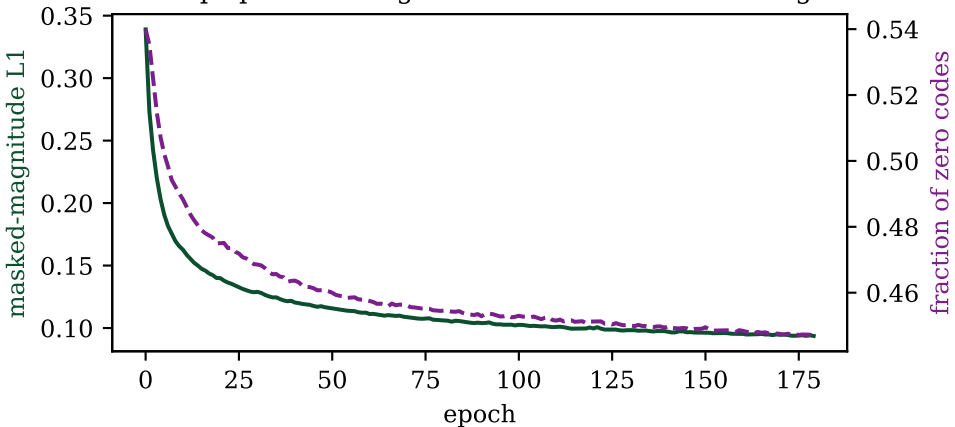
Deep sparse coding network: end-to-end training
