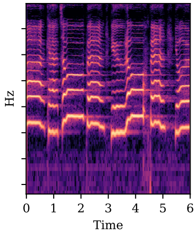
Vocals X_v
