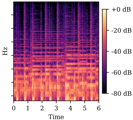
Accompaniment X_a
