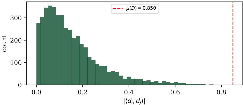
K-SVD vocal dictionary coherence (L7: exact recovery for S < 1.1 )
