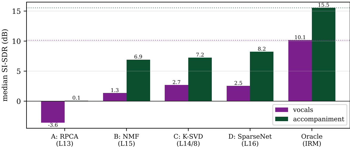
Separation quality by stage (MUSDB18 sample test)
