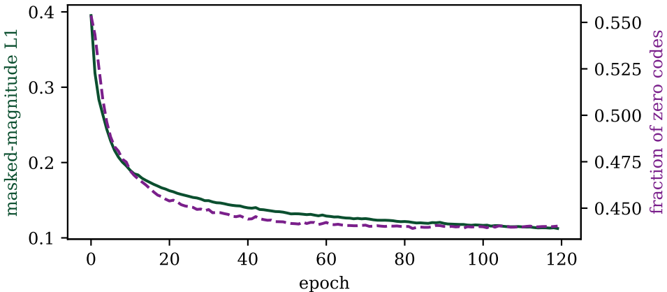
SparseNet end-to-end training (L16)
