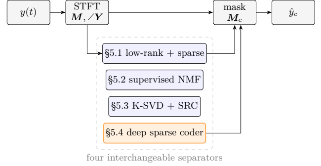
Figure 1. The shared pipeline. All four methods estimate the same time-frequency mask \mathbf{M}_c on one STFT front end and differ only in how they impose structure; resynthesis reuses the mixture phase.
