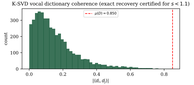
Figure 10. Off-diagonal coherence of the learned K-SVD vocal dictionary. The worst-case recovery bound certifies only s \lesssim 1 , but separation at s=10 works, evidence of an average-case-versus-worst-case gap.
