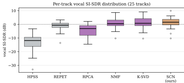
Figure 2. Per-track vocal SI-SDR over the 25 test tracks. Boxes span the interquartile range; the deep model shifts the full distribution, not only the median.
