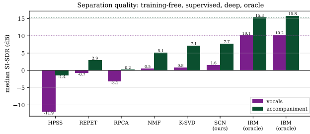
Figure 5. Median SI-SDR by method. Dotted lines mark the oracle ceilings. Supervision and unrolled learning each add a clear increment over the training-free baselines.
