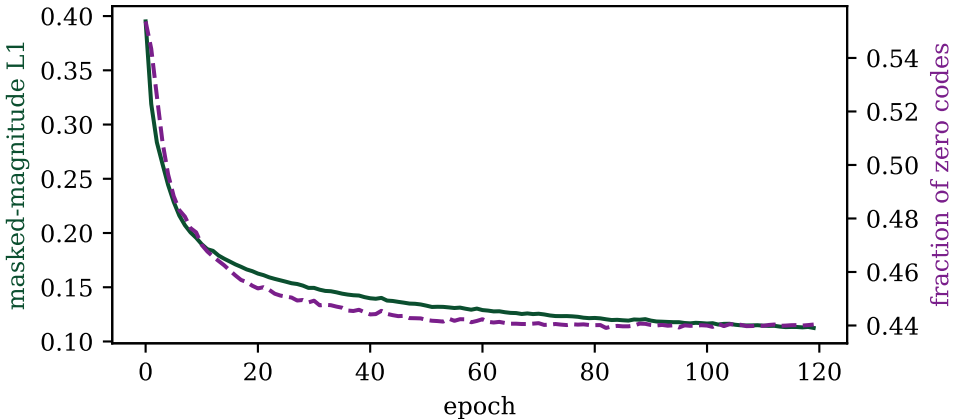
Deep sparse coding network: end-to-end training
