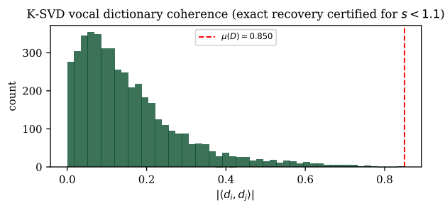
Figure 6. Off-diagonal coherence of the learned K-SVD vocal dictionary. The worst-case recovery bound certifies only s \lesssim 1 , but separation at s=10 works, evidence of an average-case-versus-worst-case gap.
