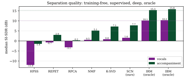
Figure 1. Median SI-SDR by method. Dotted lines mark the oracle ceilings. Supervision and unrolled learning each add a clear increment over the training-free baselines.
