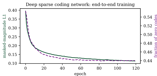
Figure 5. Deep sparse coding network training. Masked-magnitude reconstruction loss (left axis) and fraction of zero codes (right axis) across epochs.
