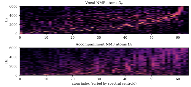
Figure 4. Supervised NMF dictionaries, atoms sorted by spectral centroid. Vocal atoms (top) versus accompaniment atoms (bottom).
