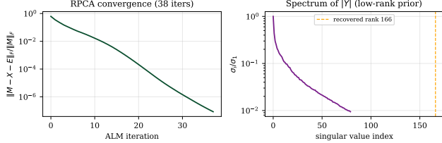
Figure 3. Left: relative residual of the principal-component-pursuit iteration. Right: normalized singular spectrum of the mixture magnitude, justifying the low-rank accompaniment prior.
