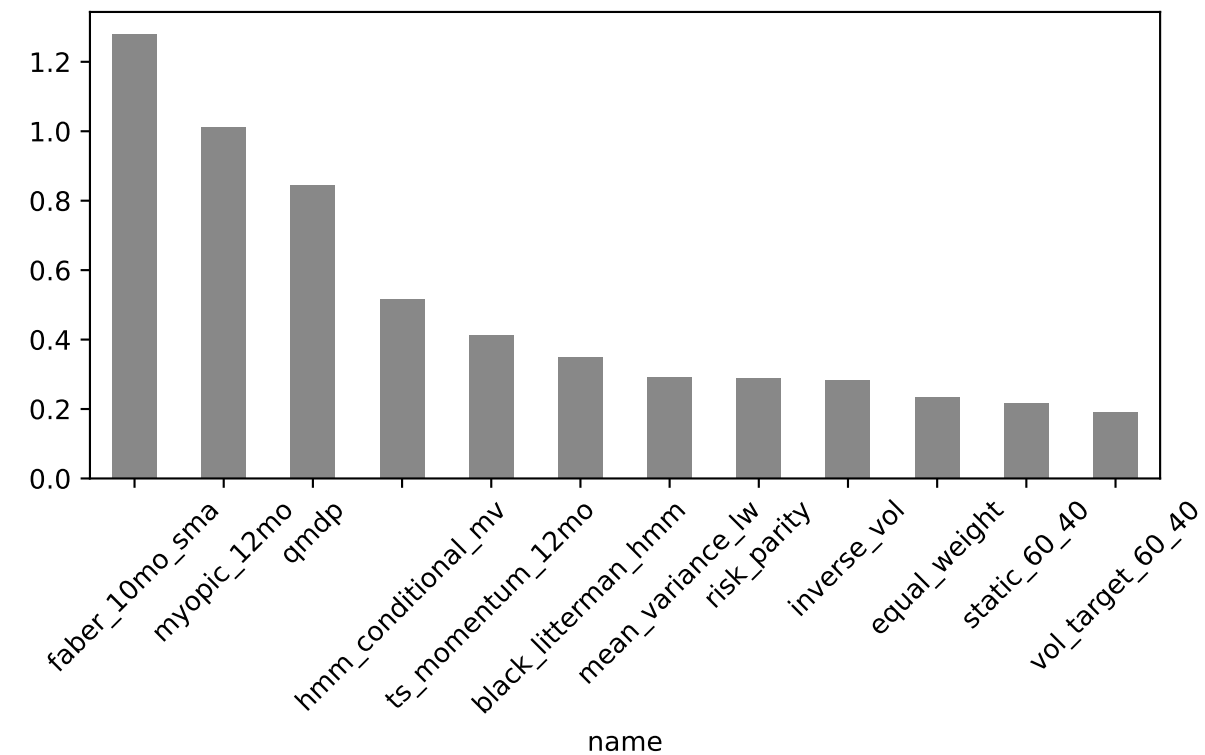
Calmar ratio
