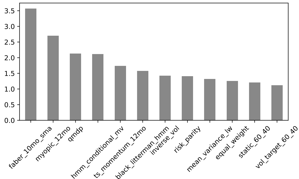
Sortino ratio
