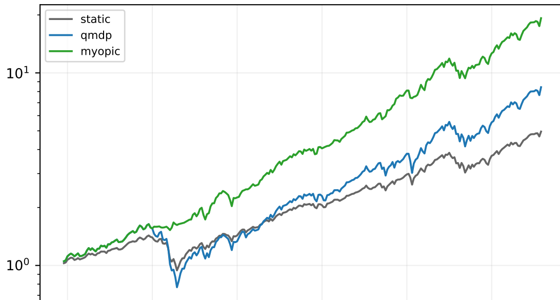
\gamma = 2.0
