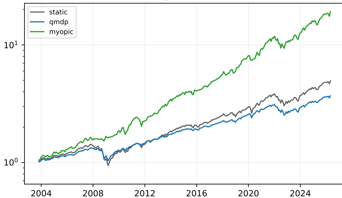
\gamma = 10.0
