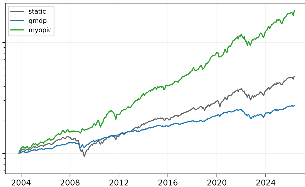
\gamma = 20.0
