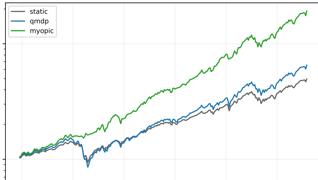
\gamma = 5.0
