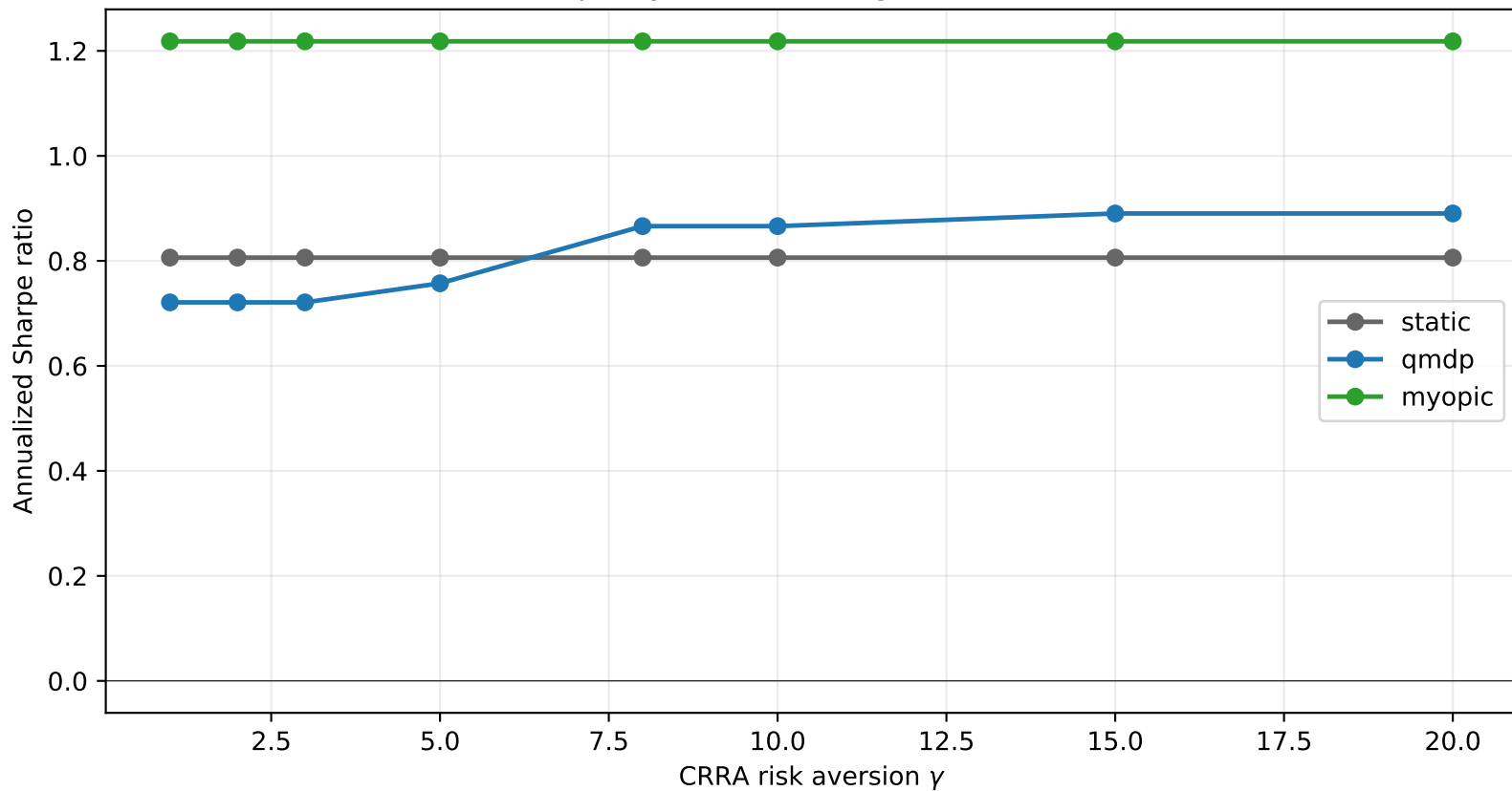
QMDP policy unlocks at higher risk aversion
