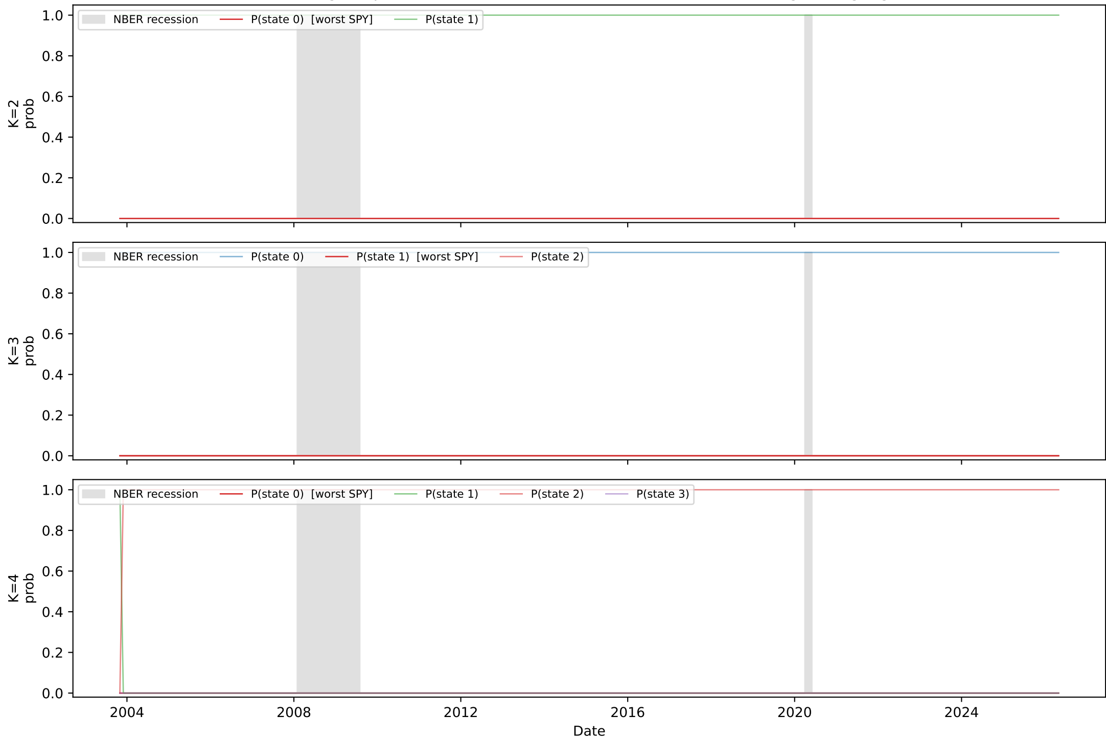
Filtered regime probabilities — 2, 3, 4-state HMMs (worst-return regime highlighted)
