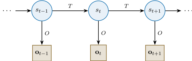
Figure 3: The Gaussian HMM as a directed graphical model. Latent regimes s_t \in \{\text{bull}, \text{bear}\} evolve via transition matrix T ; each emits an observation \mathbf{o}_t = (\text{VIX}_t, \text{spread}_t) via O(\mathbf{o} | s) = \mathcal{N}(\mu_s, \Sigma_s) . Baum–Welch maximises the marginal likelihood \sum_{s_{1:T}} p(\mathbf{o}_{1:T}, s_{1:T} | \theta) via EM with forward–backward messages.
