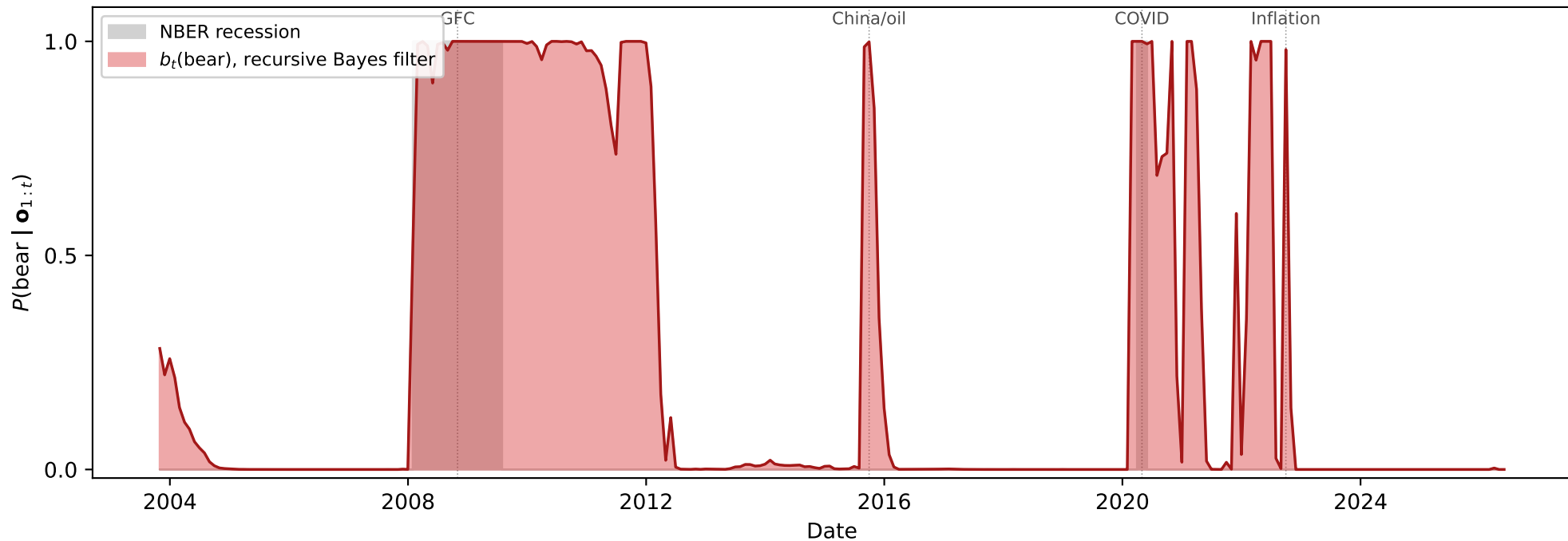
Recursively-filtered belief over the latent regime (canonical 2-state HMM, VIX + term spread)
