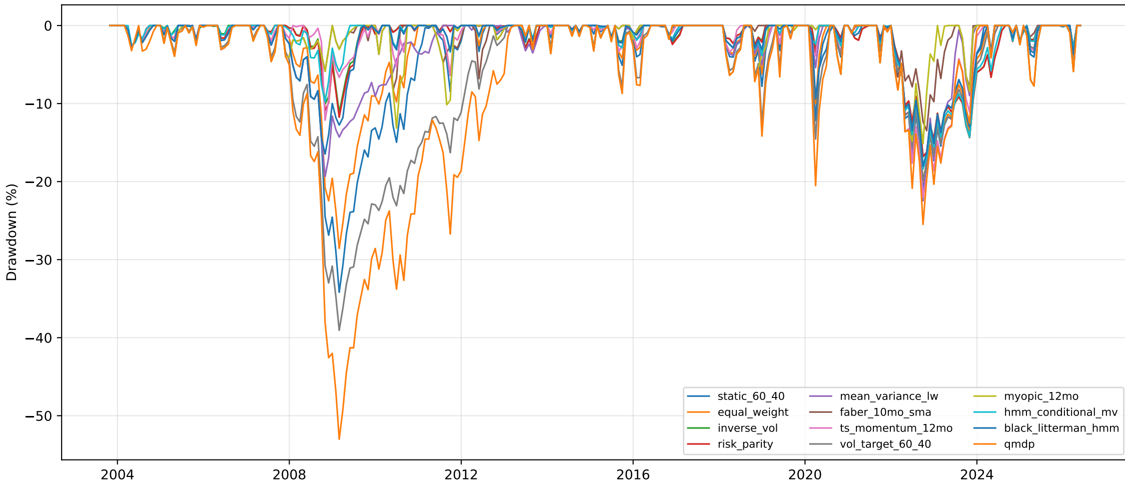
Drawdown timeseries — all baselines
