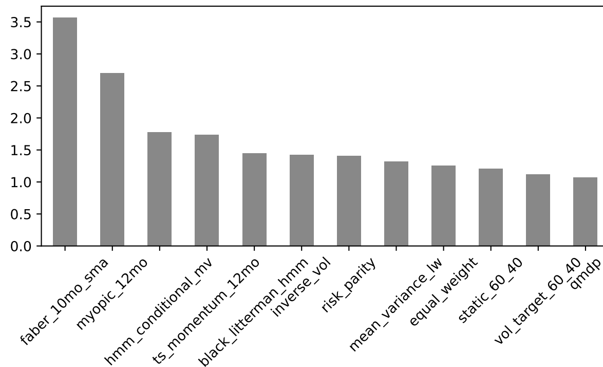
Sortino ratio
