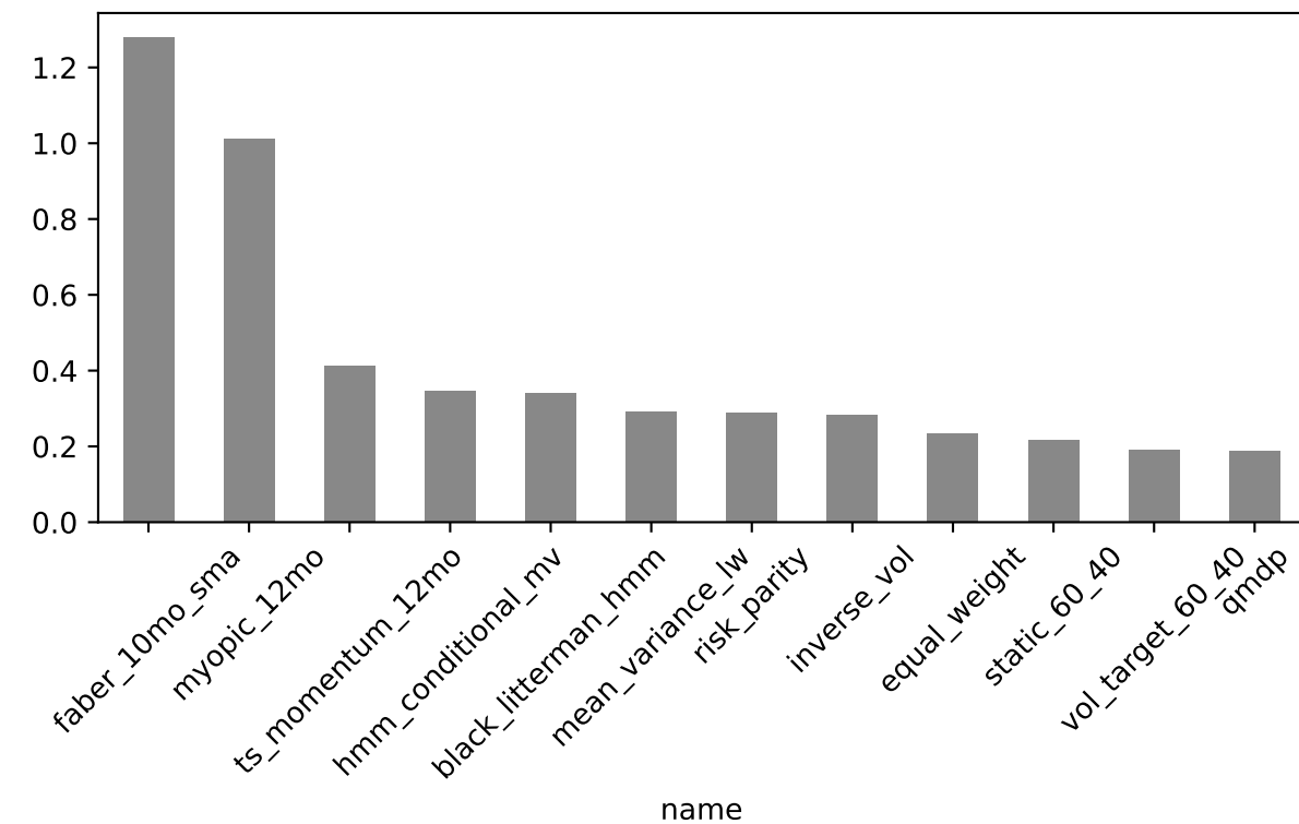
Calmar ratio
