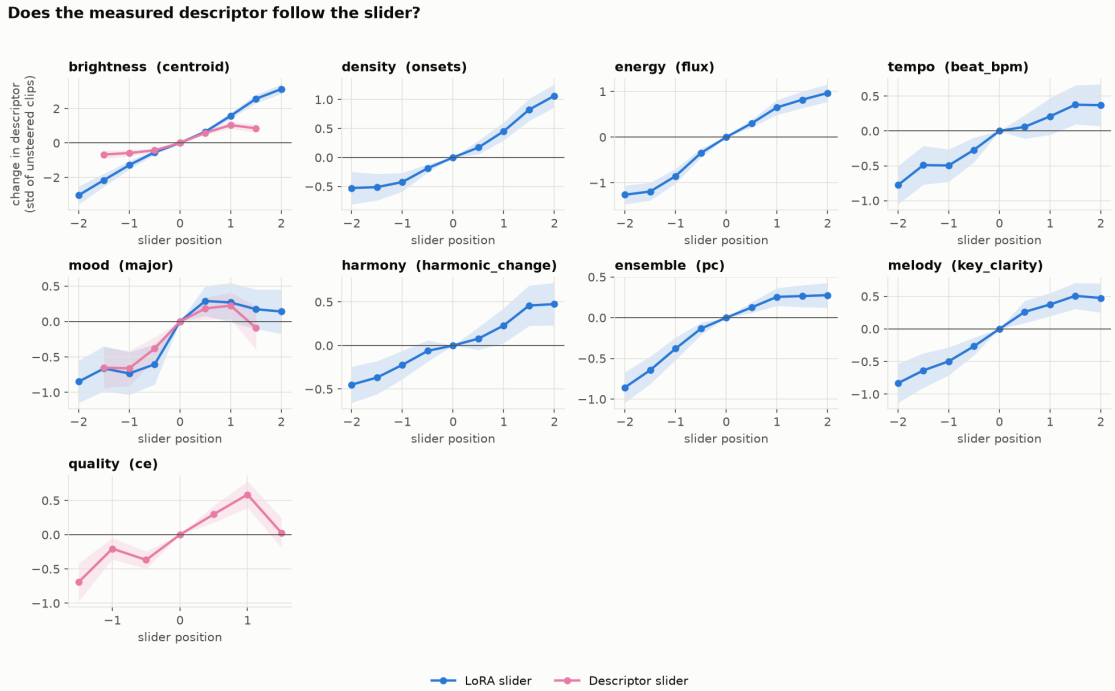
Figure 1. ACE-Step: change in each slider’s descriptor against position, in standard deviations of unsteered clips, for prompt-pair sliders and for sliders trained between two sets of clips.
