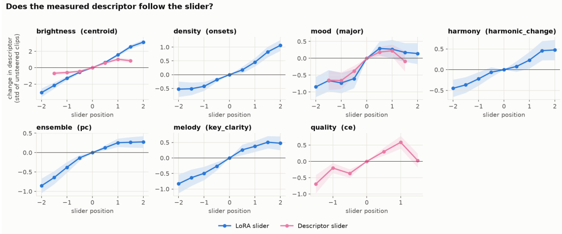
Figure 1. ACE-Step: change in each slider’s descriptor against position, in standard deviations of unsteered clips, for prompt-pair sliders and for sliders trained between two sets of clips.
