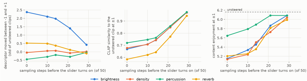
Figure 3. Timestep gating on Stable Audio Open for four sliders.
