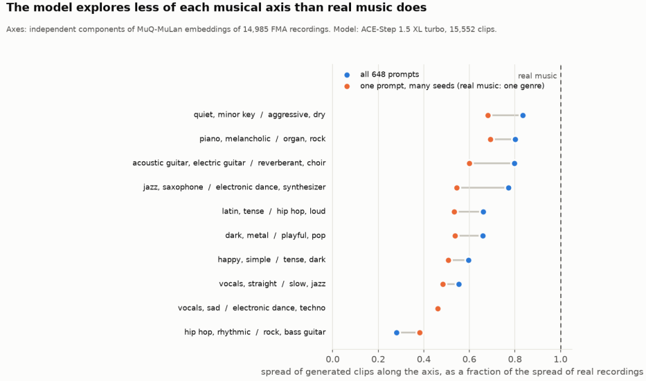
Figure 2. Coverage of ten real-music axes by 15,552 ACE-Step clips. Each axis is labelled by the tags at its two ends.
