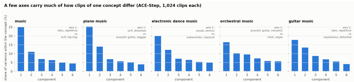
Figure 4. Share of within-concept variance carried by the first six components.
