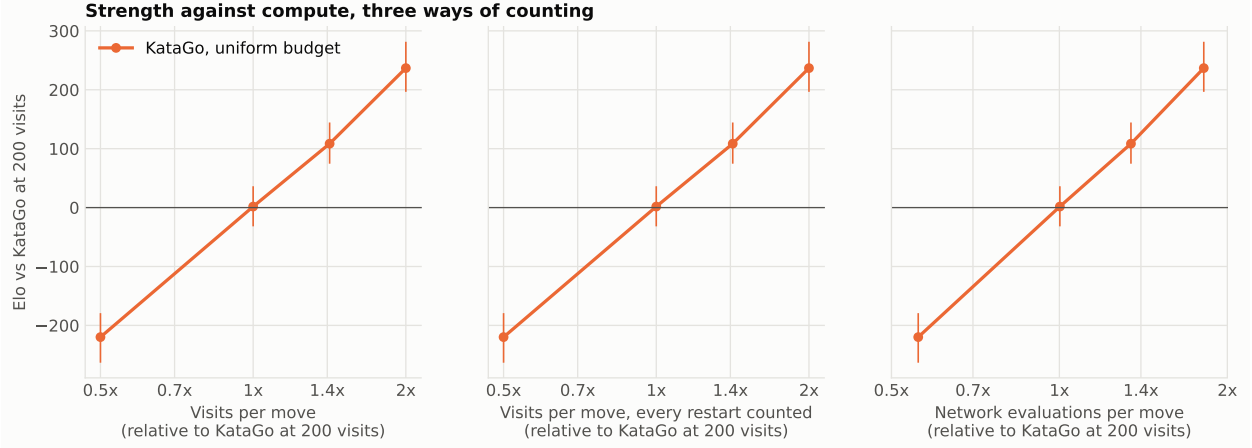
Figure 1: Elo against KataGo at 200 visits, as a function of compute relative to that baseline, counted three ways. The line is KataGo at uniform budgets. Bars are 95% intervals.
