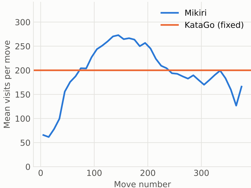
Visits by move number
