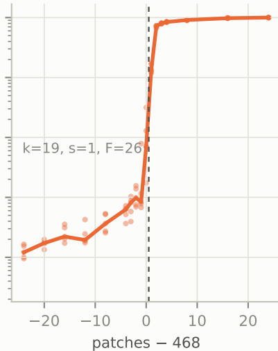
DeepSpeech-1, context 9
