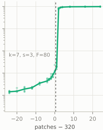
Transformer-CTC conv
