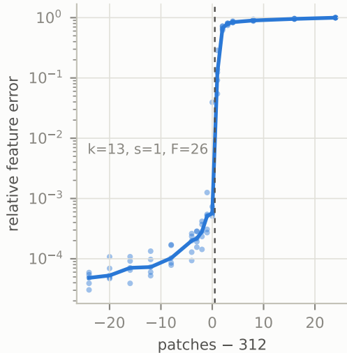
DeepSpeech-1, context 6
