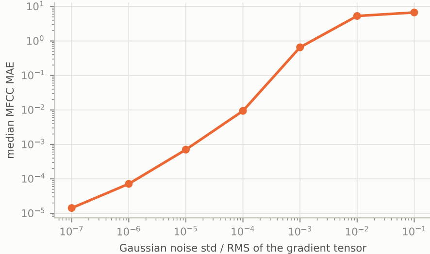
DeepSpeech-1, utterances up to 6.2 s
