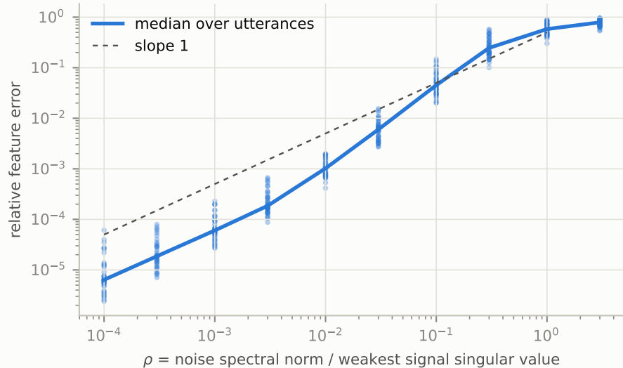
Noise hides the span when it reaches the weakest direction
