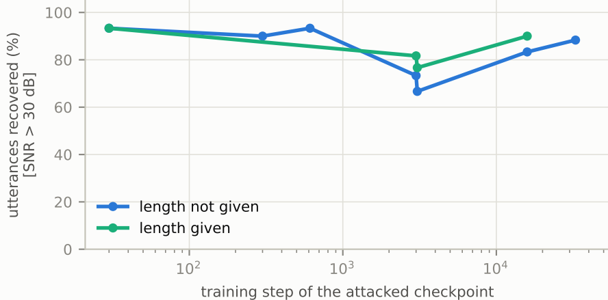
Attack success at each checkpoint
