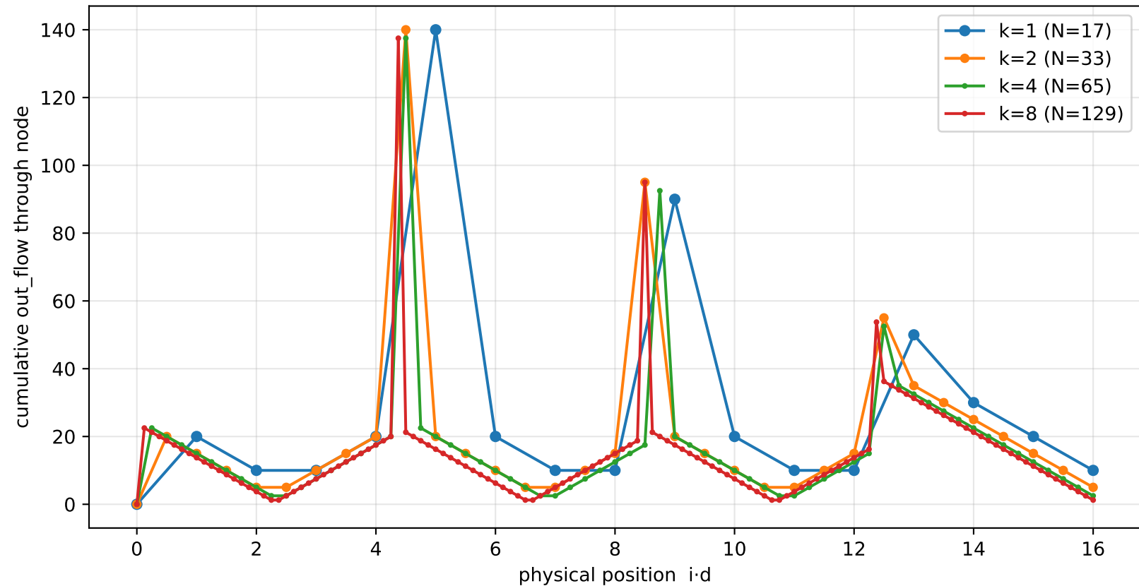
Flow profile under spatial refinement ( \phi=10 , \rho=5 , t=1 ; case d-like)
